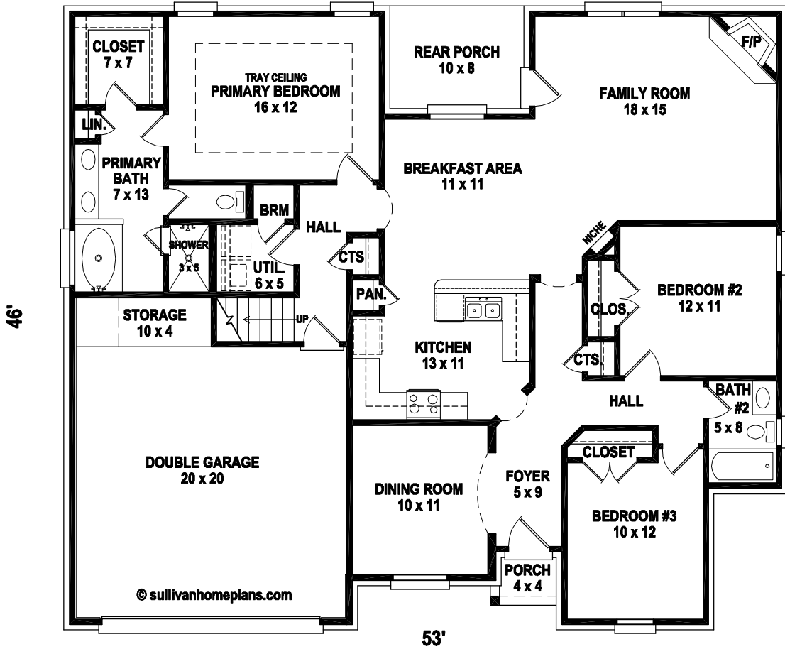
FIRST LEVEL FLOOR PLAN
